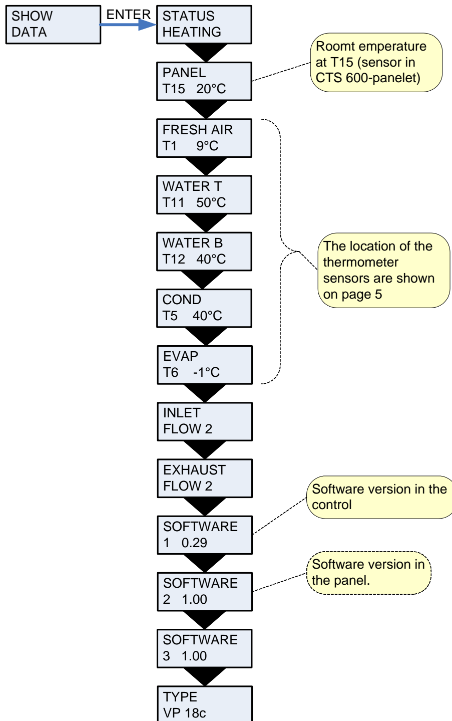
Figure 8: The "Show data" menu
