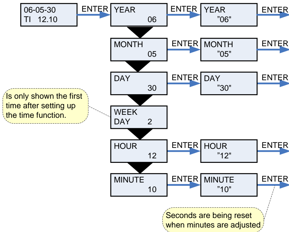
Figure 10: Setting of clock
