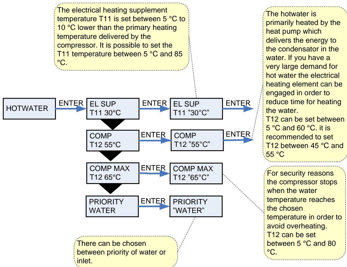
Figure 12: The "Hotwater" menu
