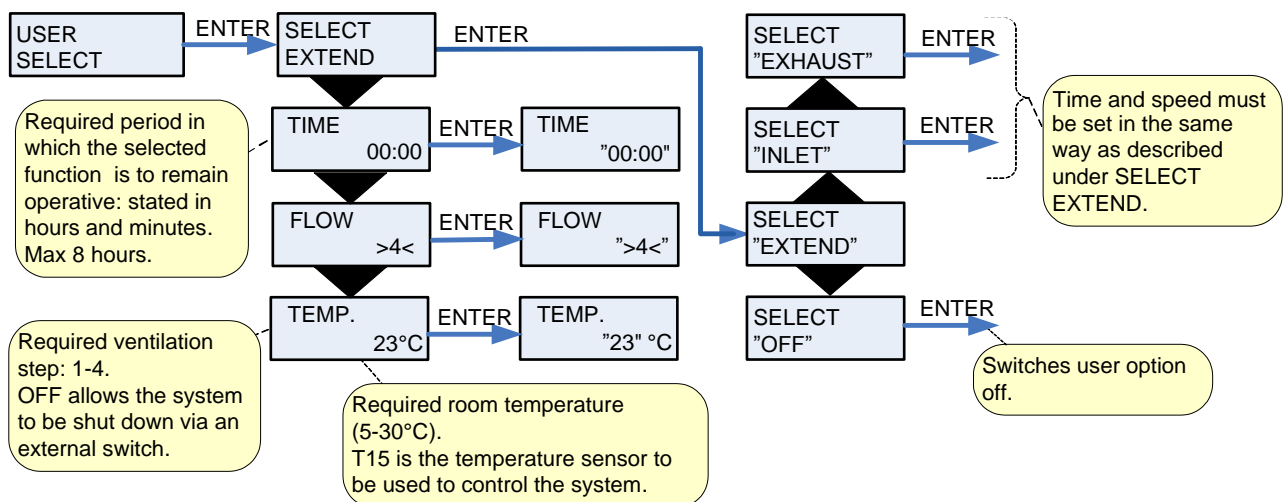
Figure 9: The "User select" menu
