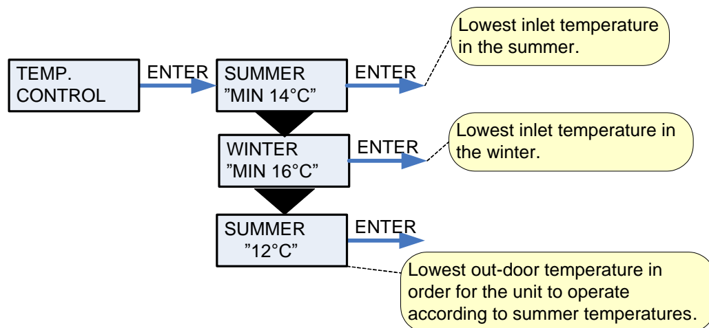
Figure 16: The "Temp. control" menu
